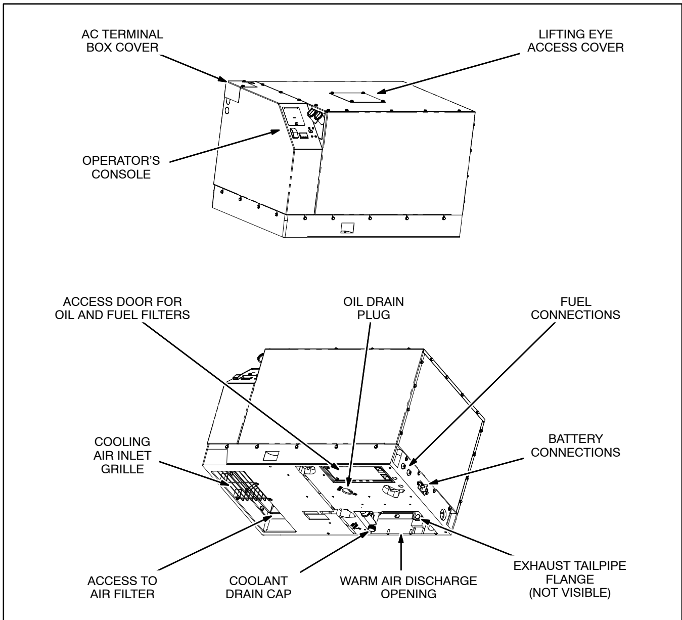
FIGURE 2. TYPICAL GENSET
